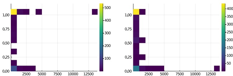
Fig. 11. Stability (left, OY axis) and groundedness (right, OY) by method size (OX) in Pluto
